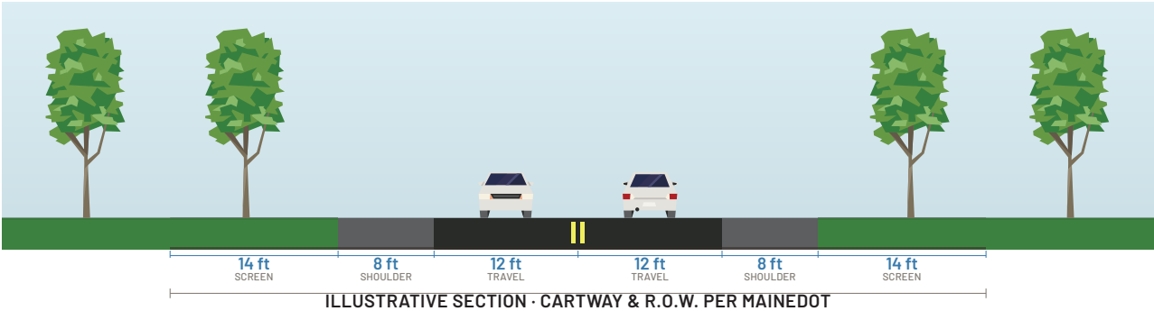
Illustrative section only. Cartway geometry and right-of-way for this Type are set by the Maine DOT (see §12); the Town governs the frontage zone, setbacks, sidewalks, and access management. Cross-section illustration adapted from Streetmix (streetmix.net), © the Streetmix project, licensed CC BY-SA 4.0.
