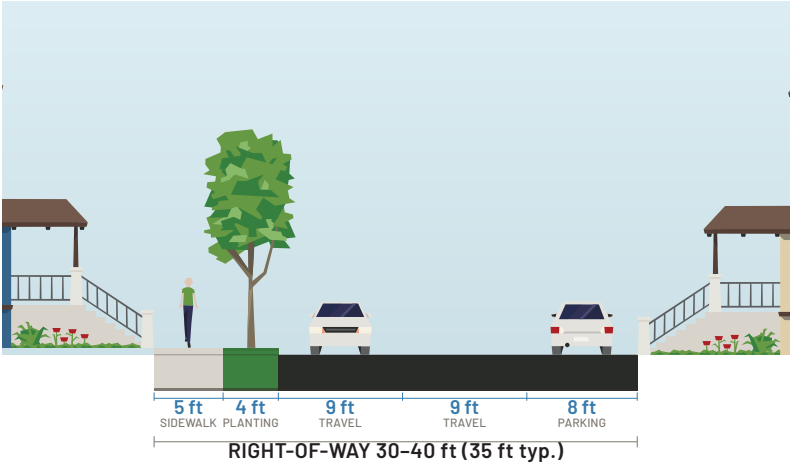
Representative section at a typical right-of-way; widths are typical values within the ranges in the Design Standards below. Cross-section illustration adapted from Streetmix (streetmix.net), © the Streetmix project, licensed CC BY-SA 4.0.
