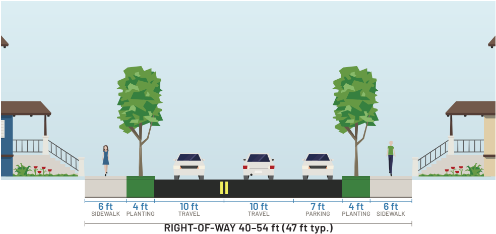
Representative section at a typical right-of-way; widths are typical values within the ranges in the Design Standards below. Cross-section illustration adapted from Streetmix (streetmix.net), © the Streetmix project, licensed CC BY-SA 4.0.
