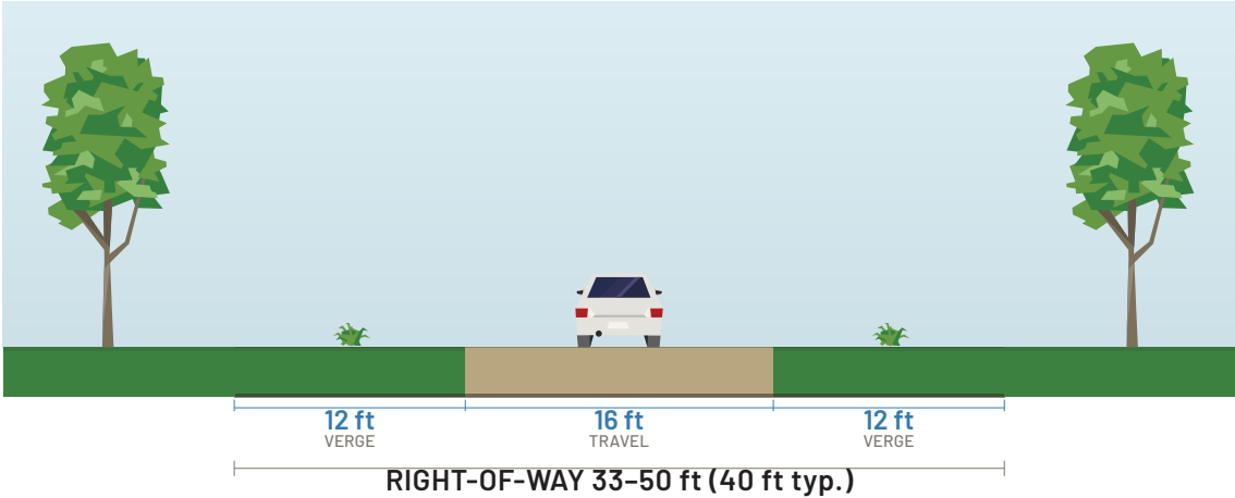
Representative section at a typical right-of-way; widths are typical values within the ranges in the Design Standards below. Cross-section illustration adapted from Streetmix (streetmix.net), © the Streetmix project, licensed CC BY-SA 4.0.
