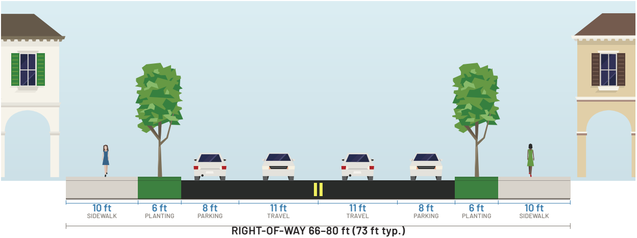
Representative section at a typical right-of-way; widths are typical values within the ranges in the Design Standards below. Cross-section illustration adapted from Streetmix (streetmix.net), © the Streetmix project, licensed CC BY-SA 4.0.
